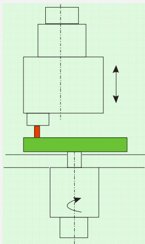
Pin on Disk test
